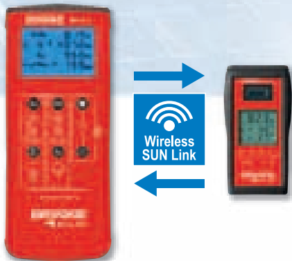
Wireless transmission of measuring data (alternatively import of measuring data by means of date/time stamp)
