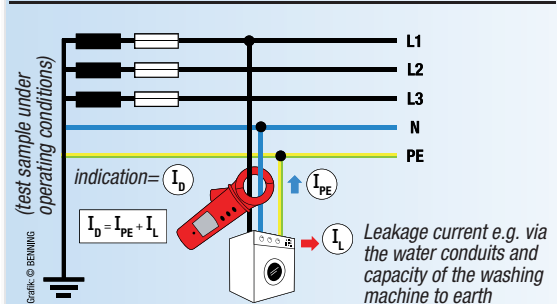
Leakage CM 9
